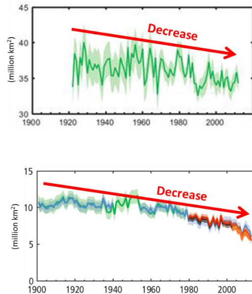
Fig. Trend in the total area of snow cover in the Northern Hemisphere (springtime) (top) Trend in the total area of sea ice in the Arctic region (summertime) (bottom)
