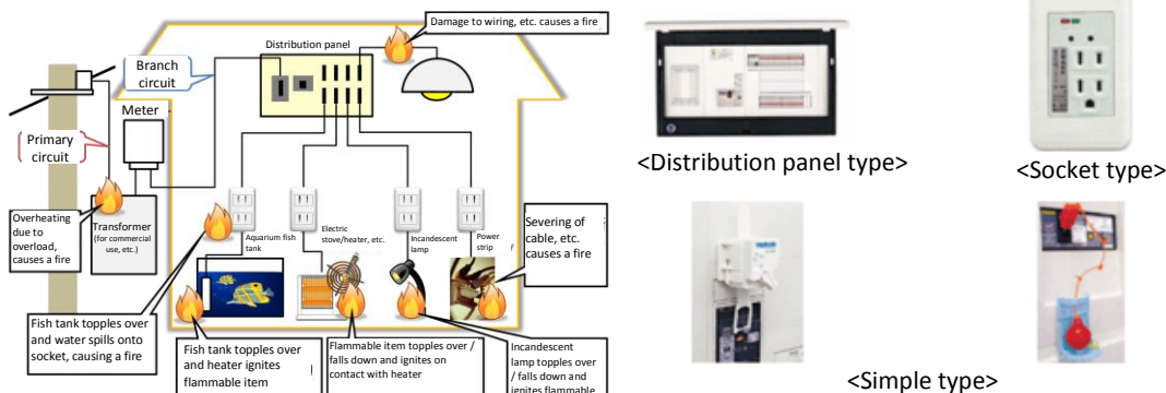
Fig. 1 Main Sites Where Electrical Fires Start Fig. 2 Examples of Earthquake-Sensitive Circuit Breakers
