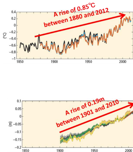
Fig. Deviations in average global surface temperature, onshore and offshore combined (top) Changes in the average global sea level (bottom)
